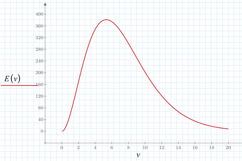
Plot of CMB Spectrum at 2.725 degrees Kelvin Vertical plot units are MJy/sr. Horizontal plot units are 1/cm
