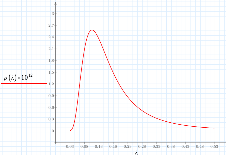
Blackbody Curve for 2.725 degrees Kelvin
